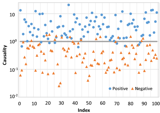
Figure 5: Distinguishing causality on ConceptNet
