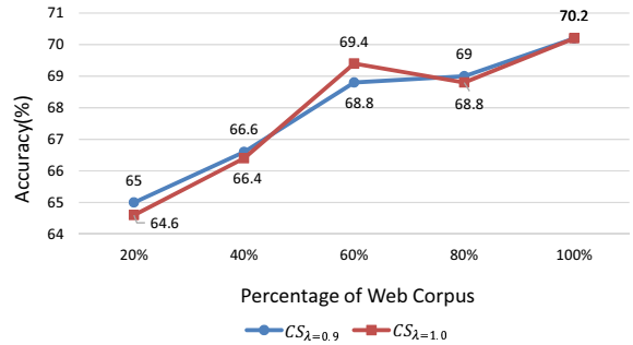
Figure 4: Distinguishing causality on ConceptNet
