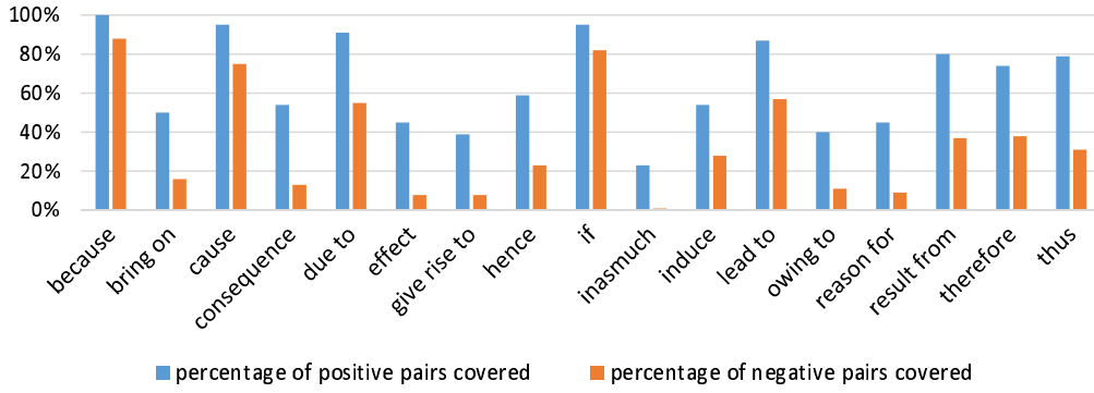
Figure 3: Number of causal vs. non-causal pairs from ConceptNet covered by cues
