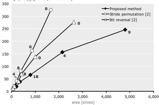
Fig. 4. Comparison of proposed general method with [2]. Labels: number of BRAMs.
