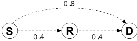
Figure 1: An example scenario to illustrate adverse selection in basic opportunistic routing. There is a session from source S to destination D , with an intermediate node R . True link loss probabilities are shown near the links.
