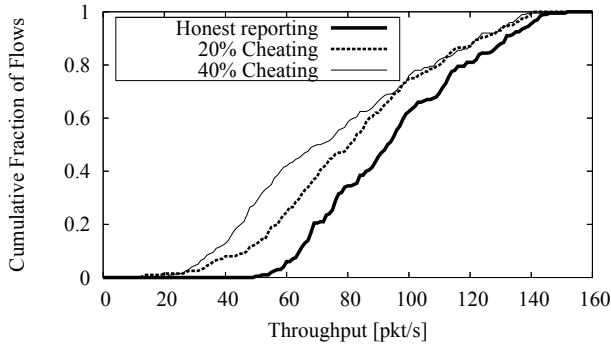
Figure 8: CDF of the unicast throughput achieved with vs. without the simple extension on 200 source-destination pairs. When the original MORE protocol is used, 20% or 40% of the nodes cheat in reporting loss probabilities.
