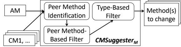
Figure 3: Overview of \text{CMSuggester}_M
