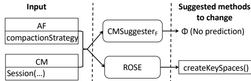
Figure 5: A task for which ROSE outperformed \text{CMSuggester}_F
