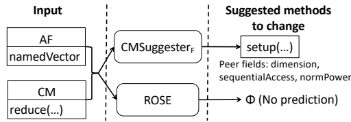
Figure 4: A task for which \text{CMSuggester}_F outperformed ROSE
